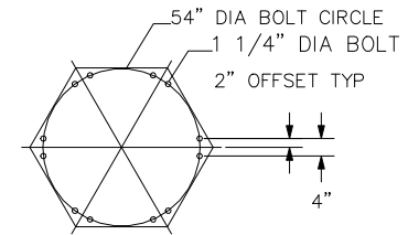
12 BOLT BASE BOLT PATTERN 1 1/4" BASE PLATE THICKNESS AT ANCHOR BOLT VIEW A-A NOT TO SCALE
