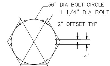
12 BOLT BASE BOLT PATTERN 1 1/4" BASE PLATE THICKNESS AT ANCHOR BOLT VIEW A-A NOT TO SCALE
