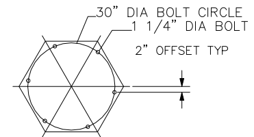
6 BOLT BASE BOLT PATTERN 1 1/4" BASE PLATE THICKNESS AT ANCHOR BOLT VIEW A-A NOT TO SCALE
