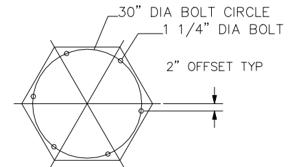
6 BOLT BASE BOLT PATTERN 1 1/4" BASE PLATE THICKNESS AT ANCHOR BOLT VIEW A-A NOT TO SCALE
